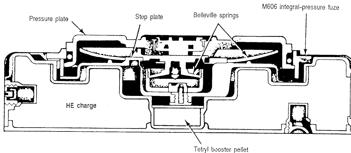
Figure A-35. M19 antitank mine
