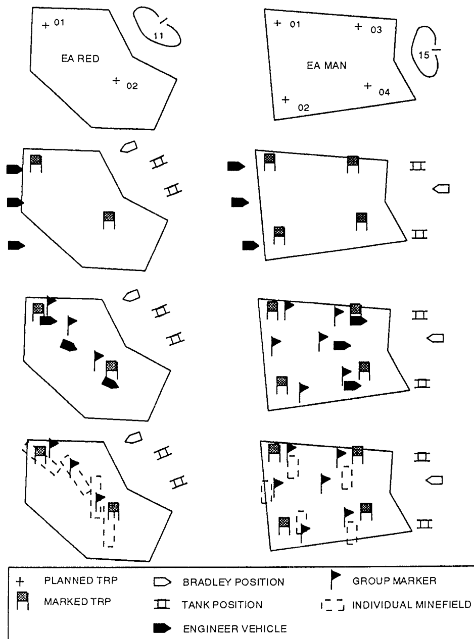
Figure 2-17. Minefield siting
