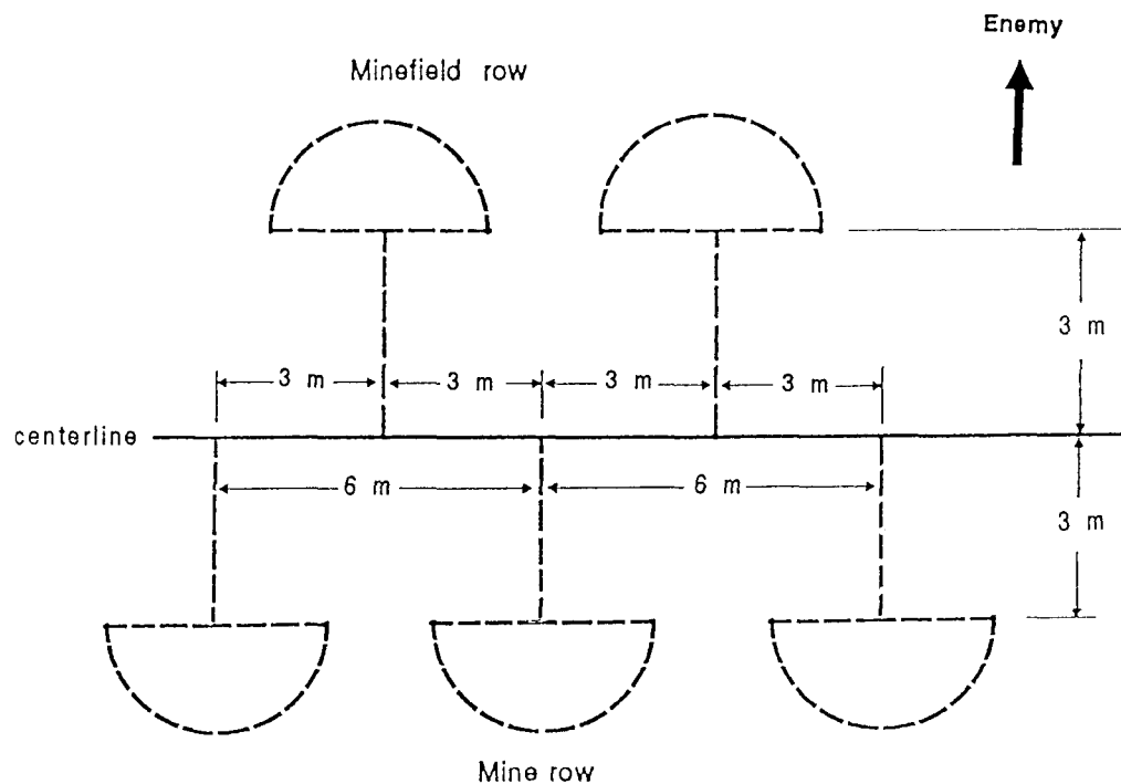
★ Figure 3-3. Arrangement of clusters in a strip
