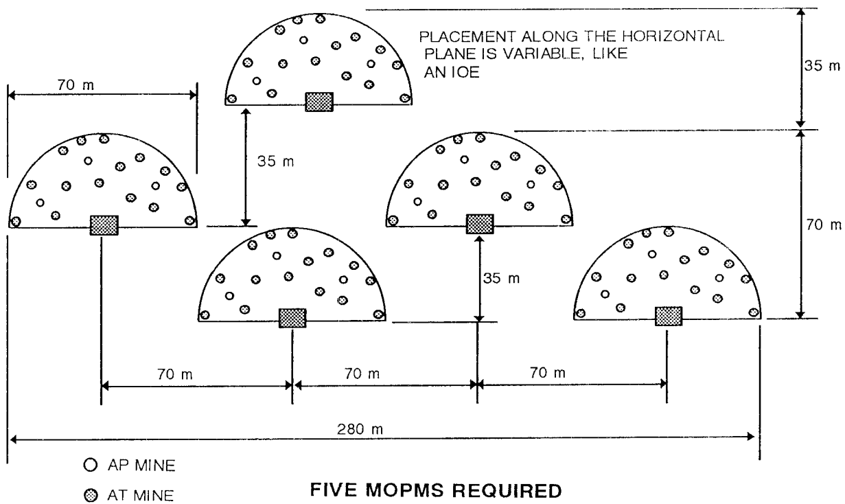
Figure 6-21. MOPMS fix minefield
