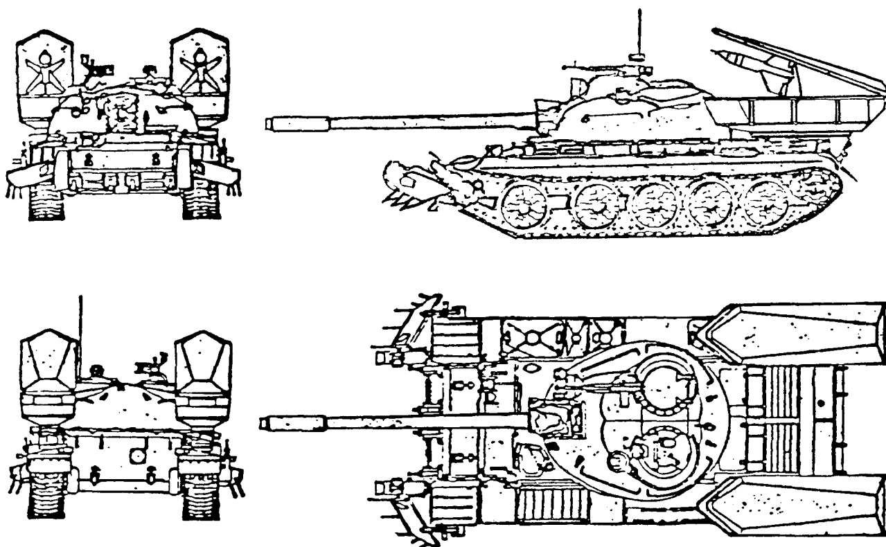
Figure C-7. KMT-4/6
