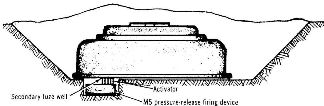
Figure 1-11. AHD incorporating a release mechanism
