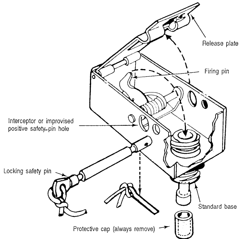
Figure A-52. M5 pressure-release firing device (mousetrap)
