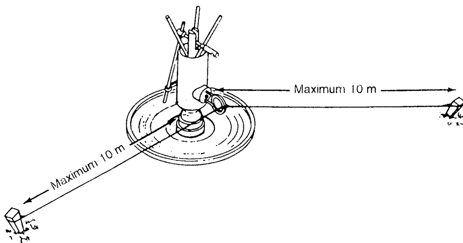
★ Figure 2-20. Trip-wire operated igniter
