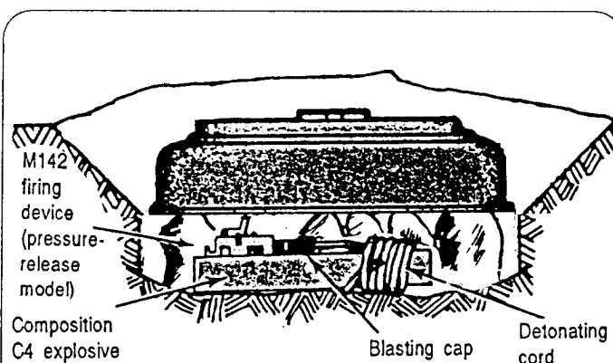
Figure 1-12. AHD not attached to mine
