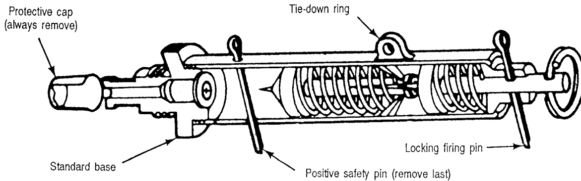
Figure A-46. M1 pull firing device
