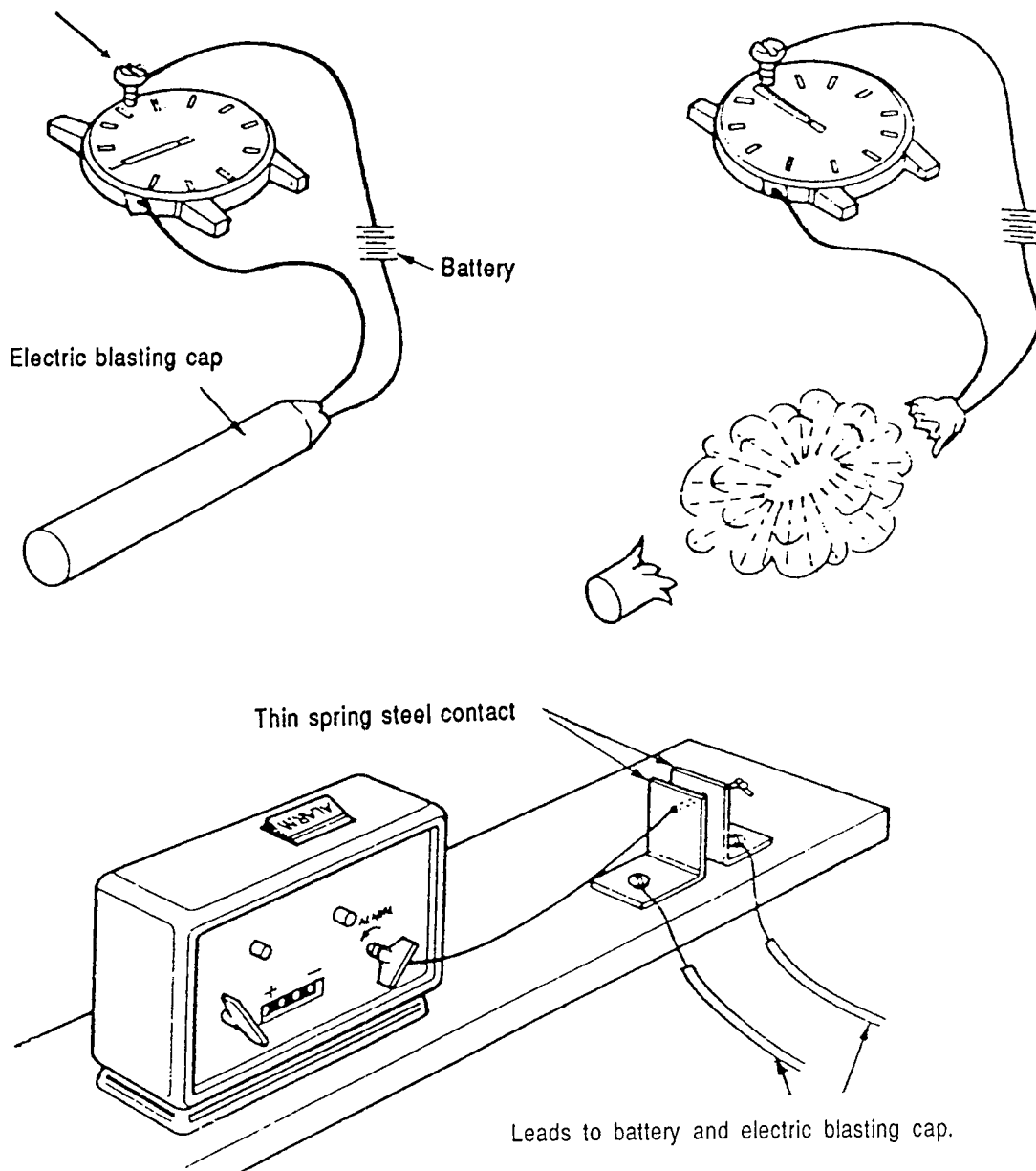
Figure 13-10. Improvised electric delay devices
