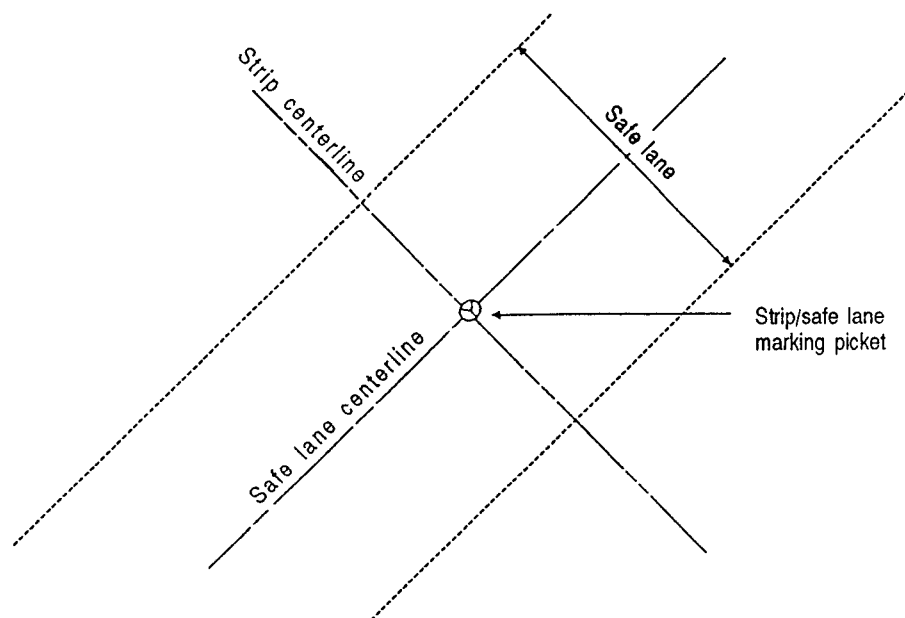
Figure 3-14. Sealing a lane - strip/safe lane marking picket
