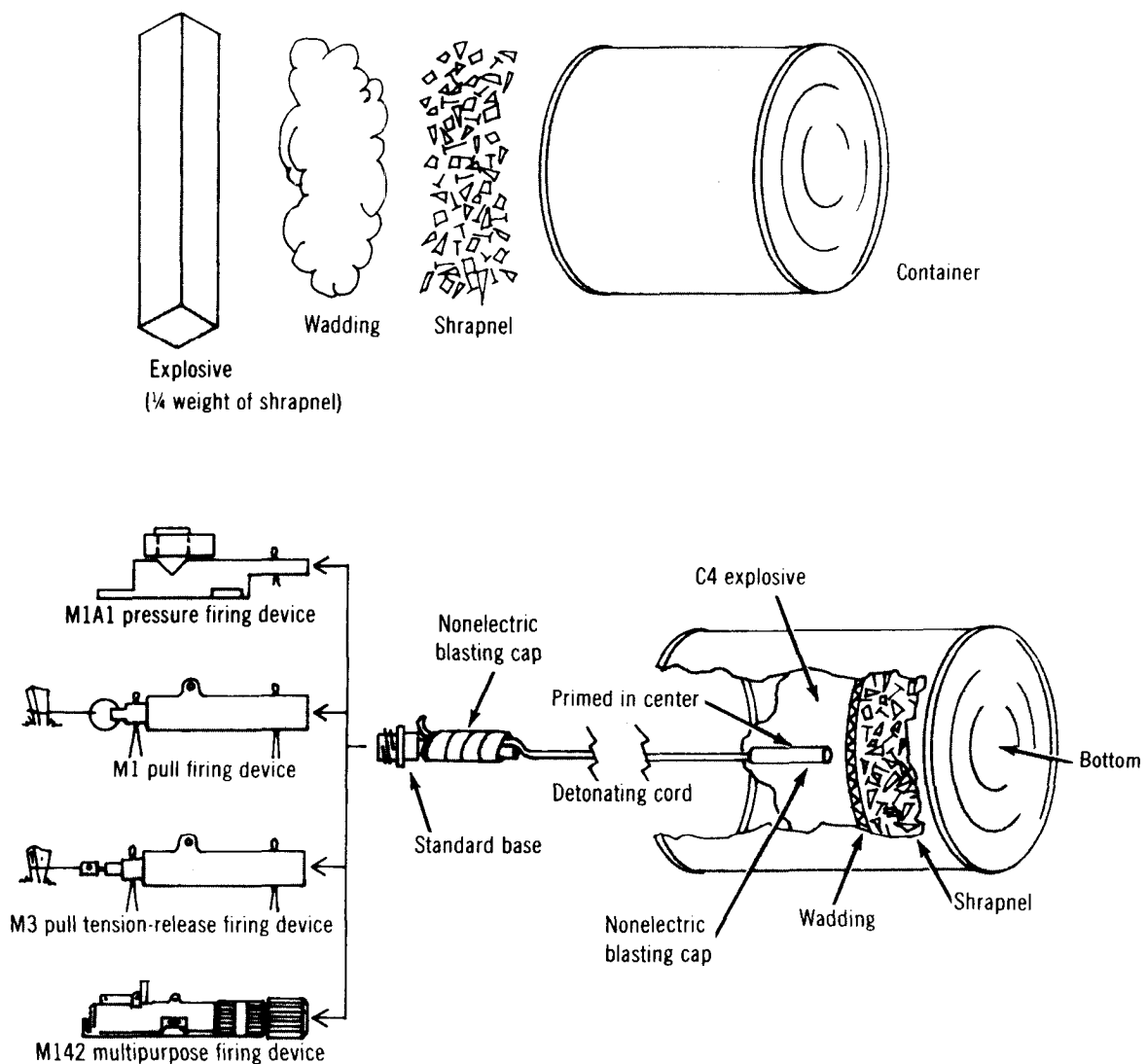
Figure 12-4. Grapeshot antipersonnel mine
