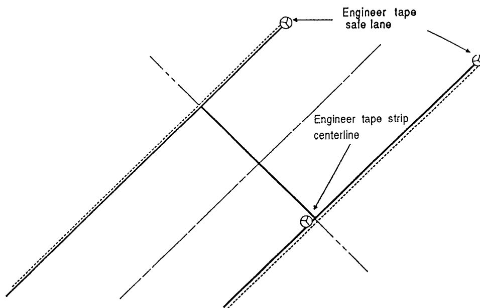
Figure 3-15. Sealing a lane - laying out the tapes
