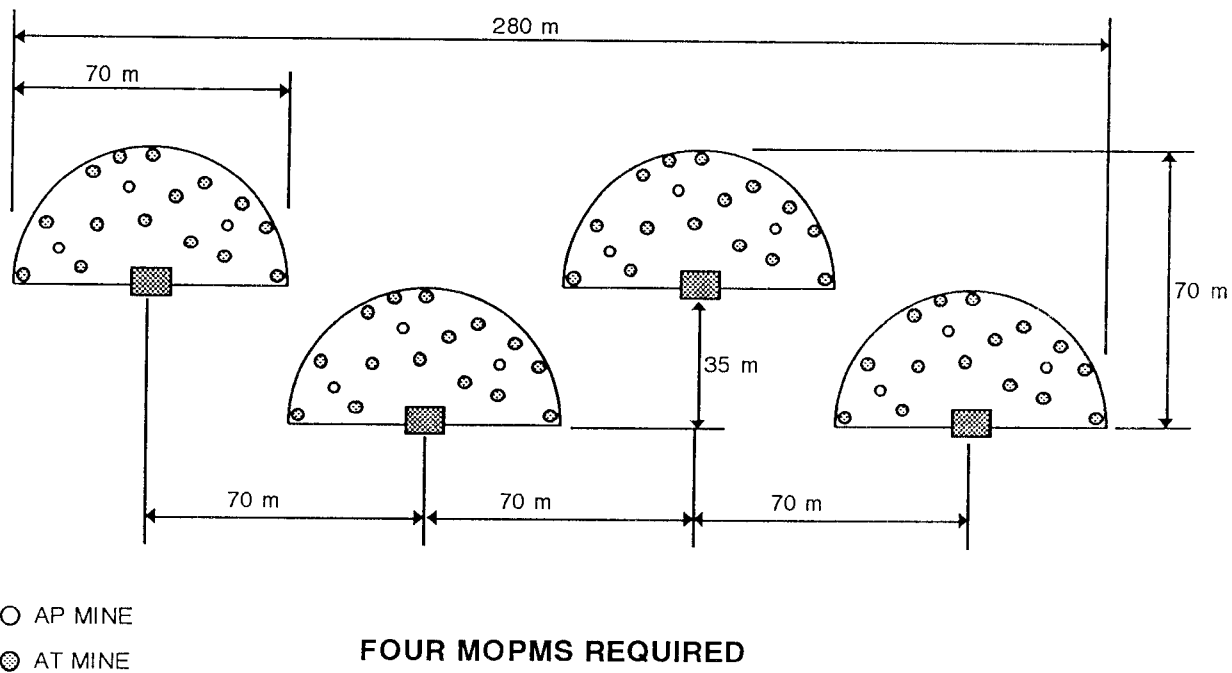
Figure 6-20. MOPMS disrupt minefield
