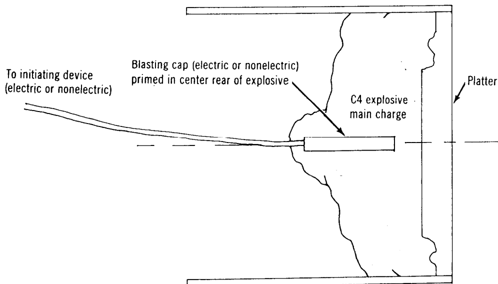
Figure 12-2. Platter charge
