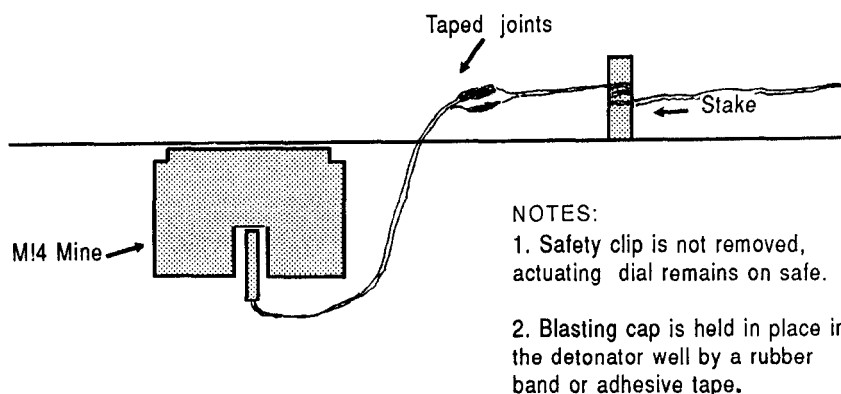
Figure E-1. M14 AP mine
