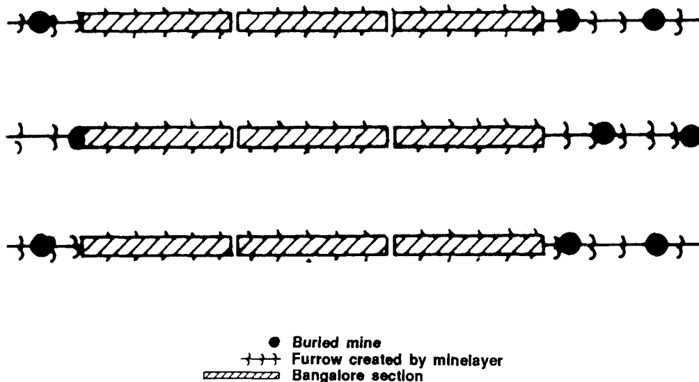
Figure 9-8. Placing bangalore sections to breach mechanically placed mines
