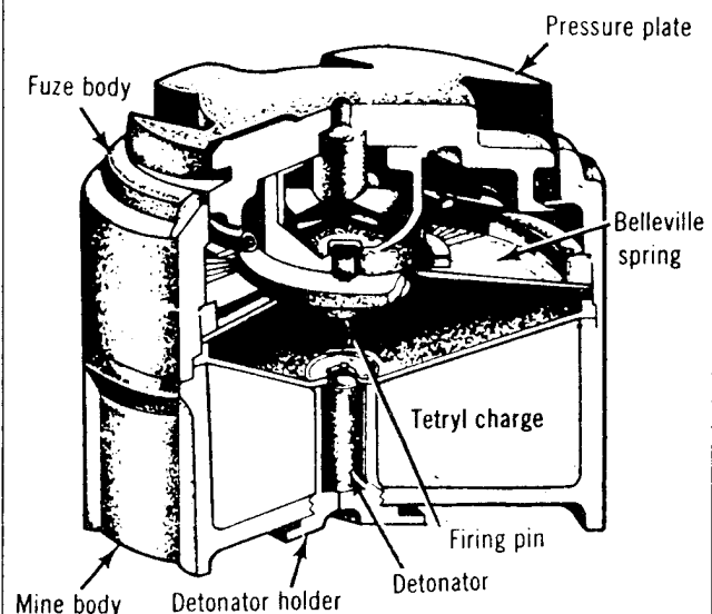
Figure A-2. M14 antipersonnel mine
