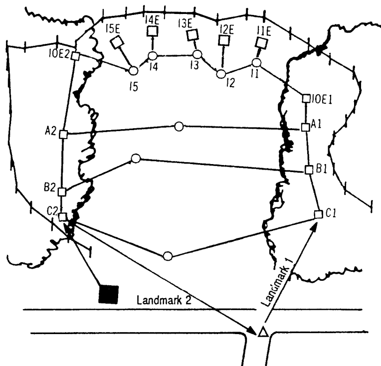
★ Figure 3-11. Stakes driven flush into the ground
