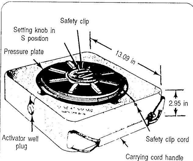
Figure A-34. M19 antitank mine
