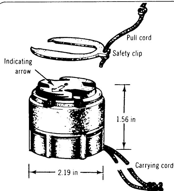
Figure A-1. M14 antipersonnel mine
