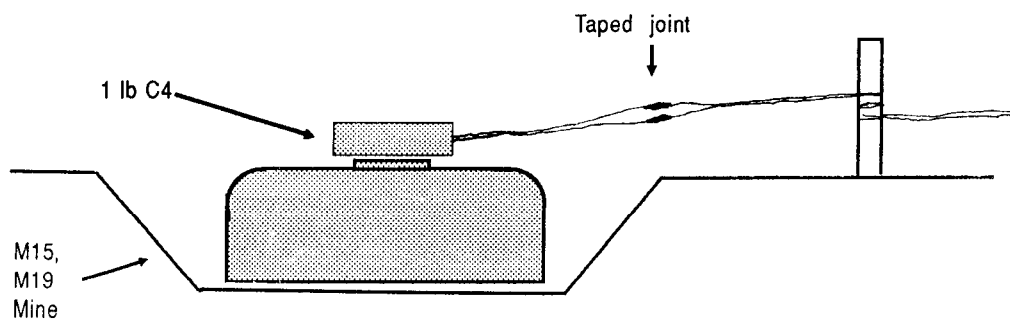
Figure E-4. M15 and M19 AT mines
