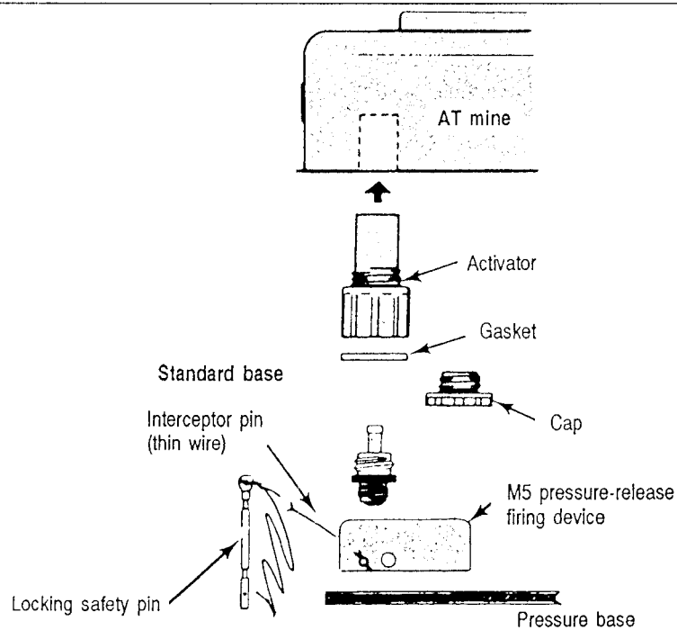
Figure A-53. M5 pressure-release firing device (mousetrap) (continued)
