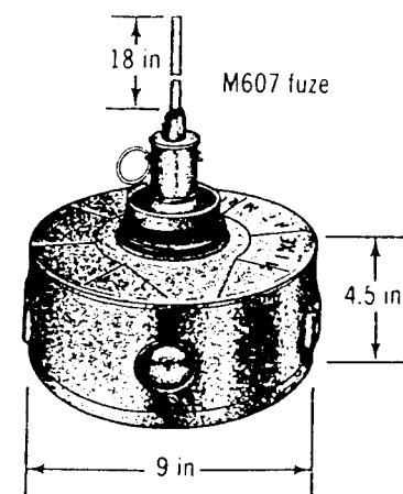
Mine, AT, HE, heavy, M21
