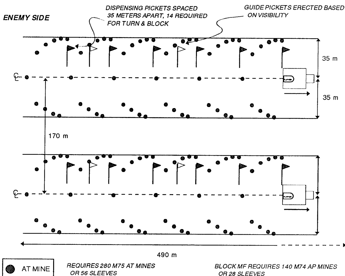
Figure 6-13. Standard Flipper turn and block minefields
