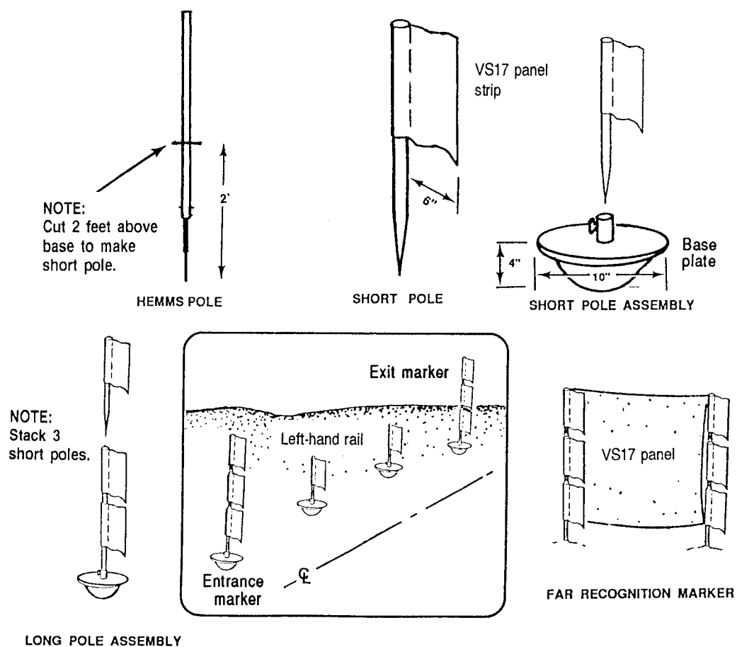
Figure 9-18. HEMMS and Tippy Tom marking combination
