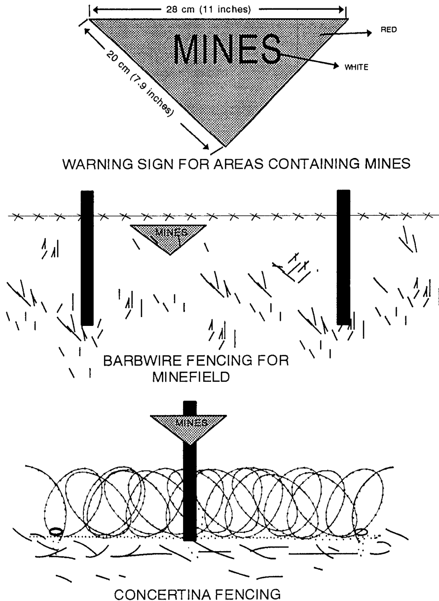
Figure 2-28. Minefield marking
