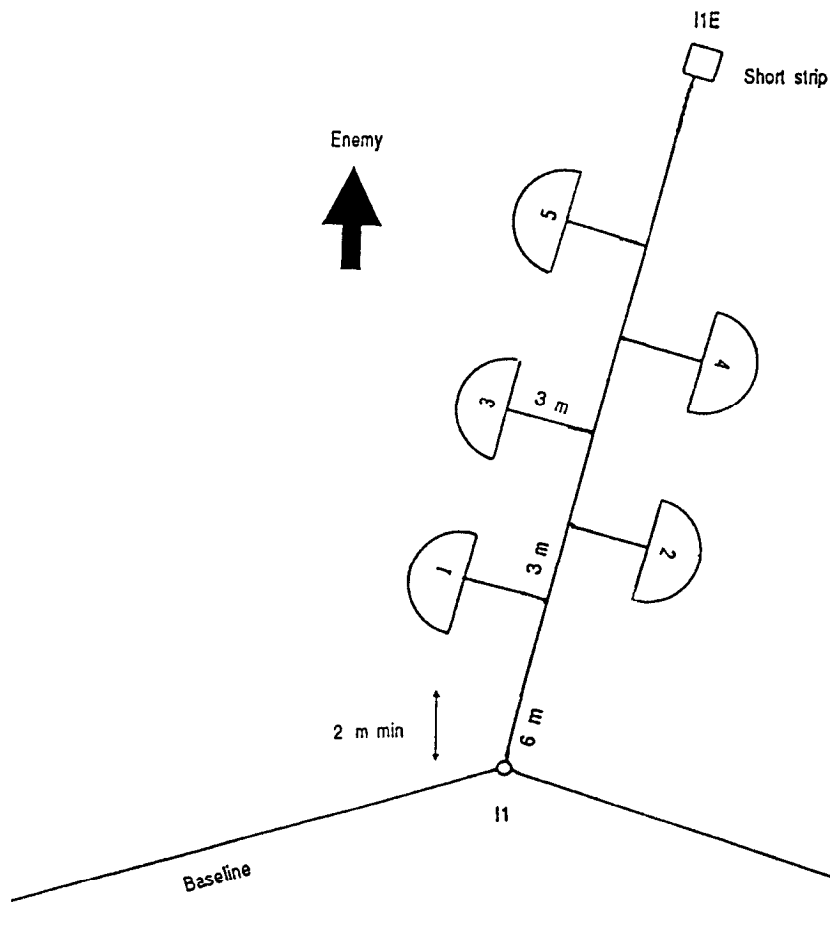
★ Figure 3-5. Clusters on short strips
