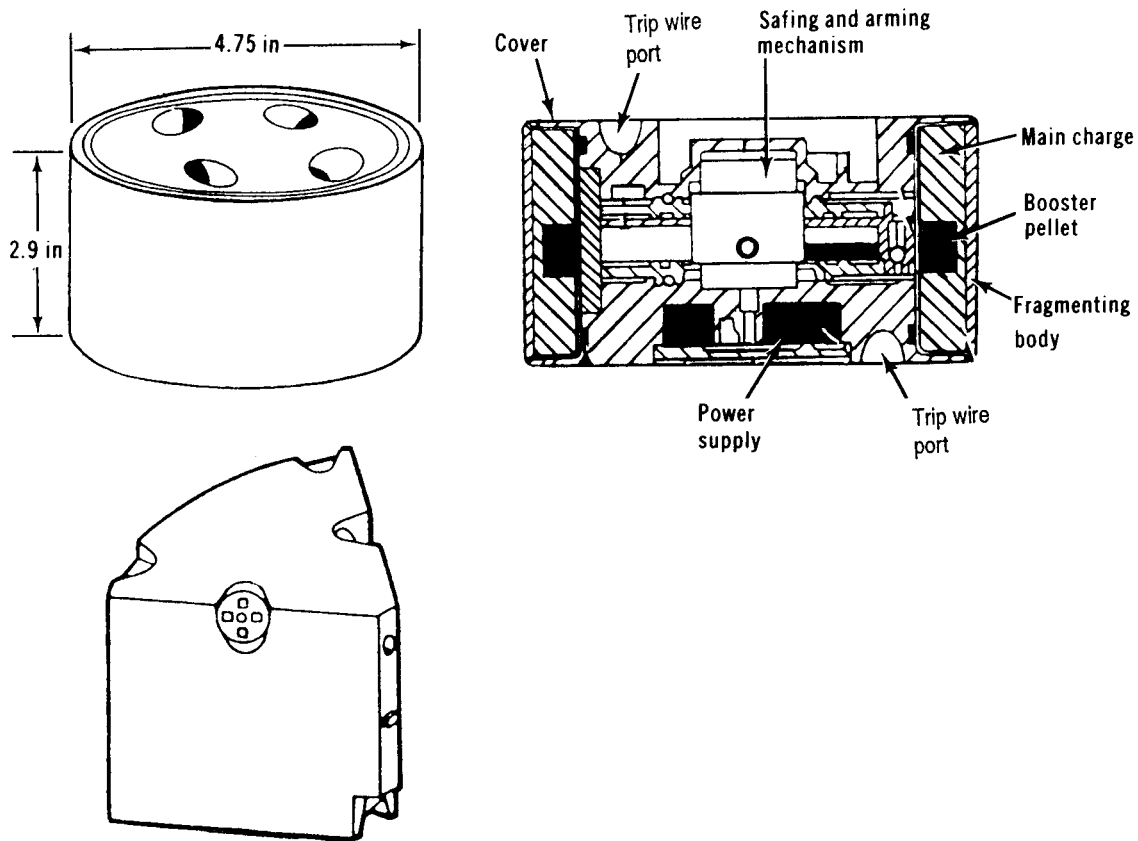
Figure 6-1. Antipersonnel mines
