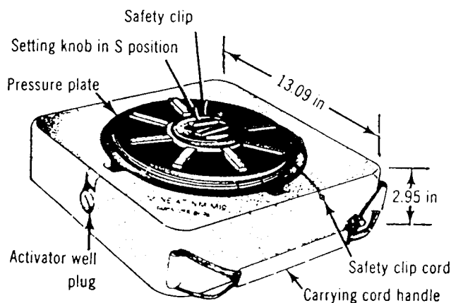
Mine, AT, HE, nonmetallic, M19
