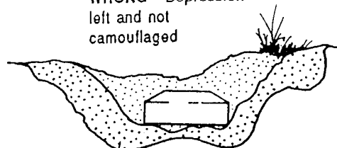
Figure 2-21. Burying and concealing mines
