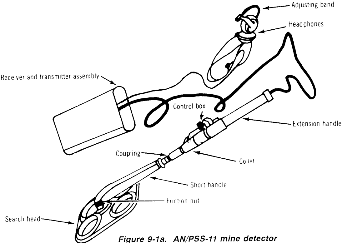
Figure 9-1a. AN/PSS-11 mine detector
