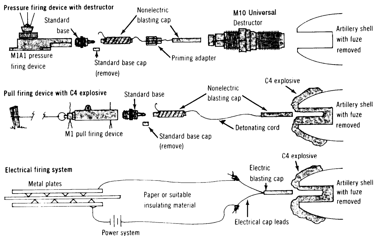
Figure 12-1. HE artillery shell antitank mine
