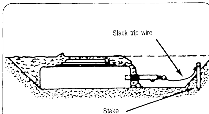
Figure A-47. M1 in the side fuze well
