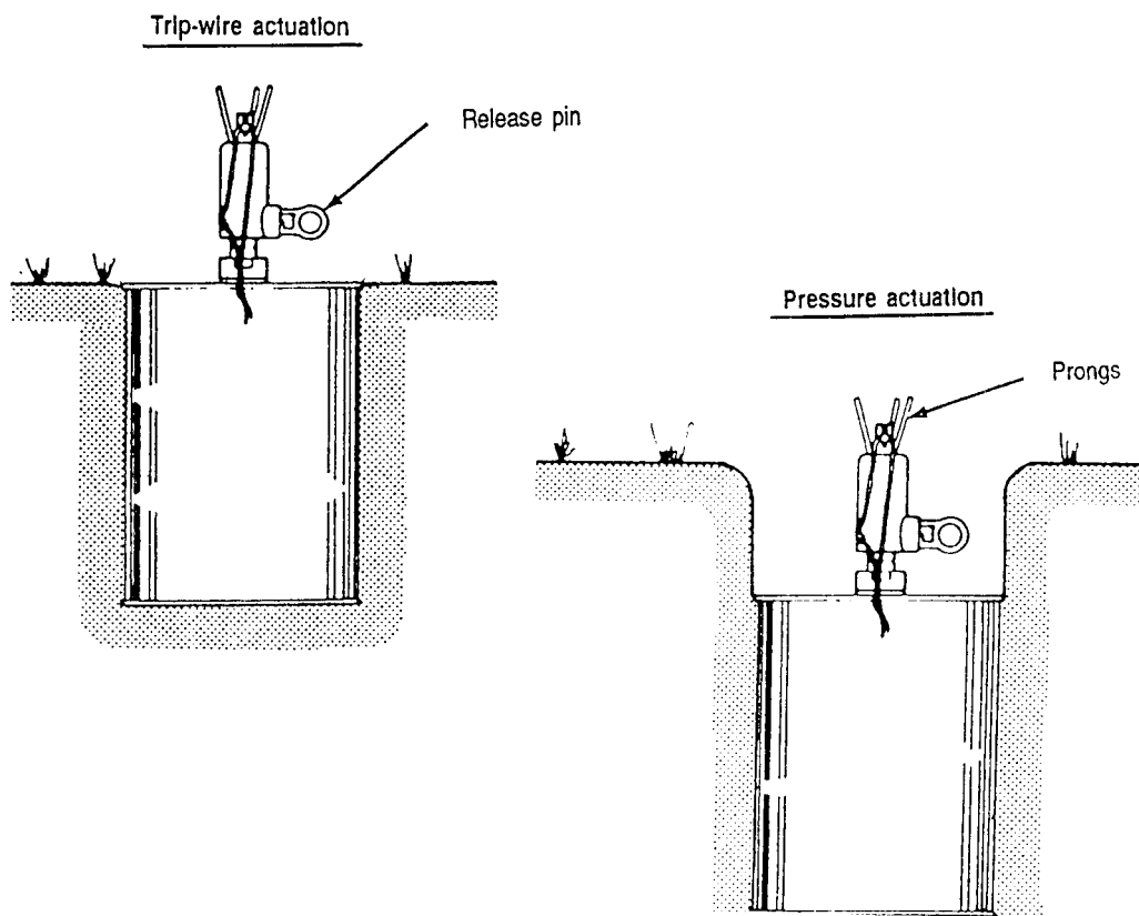
★ Figure 2-19. Prong or stud-operated igniter
